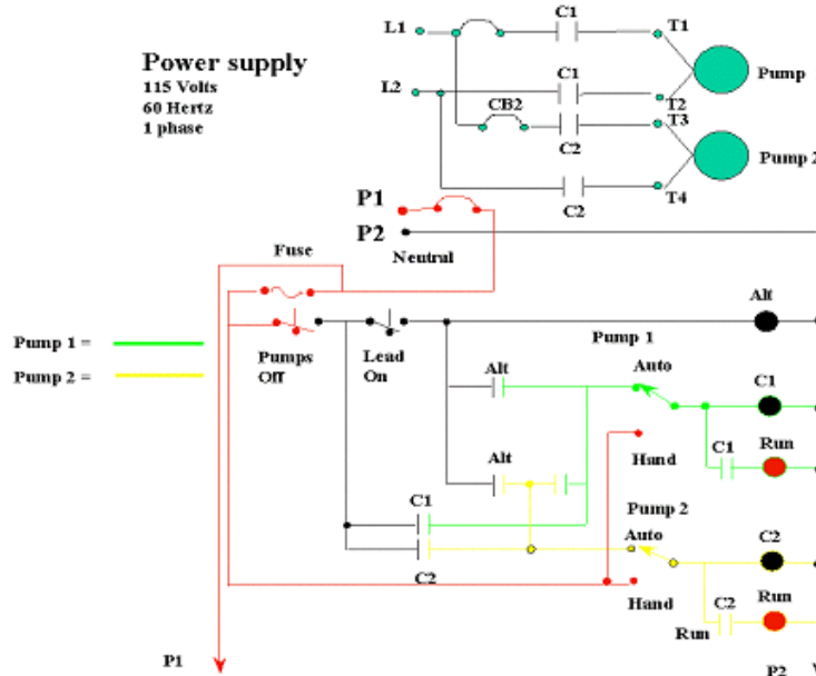
Figure 35: Duplex Pump Control Circuit
