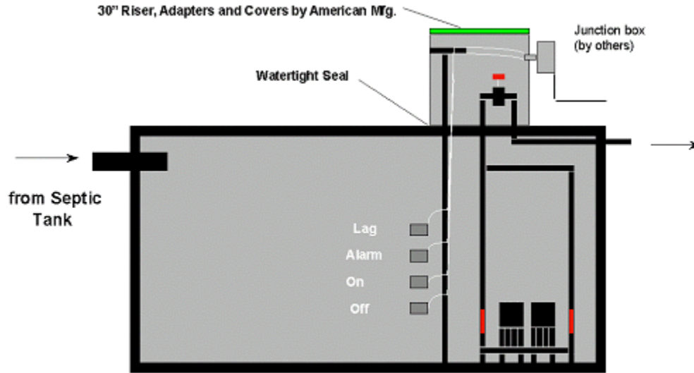
Figure 74: Duplex 4 float control system as it would be installed in a pump tank.
