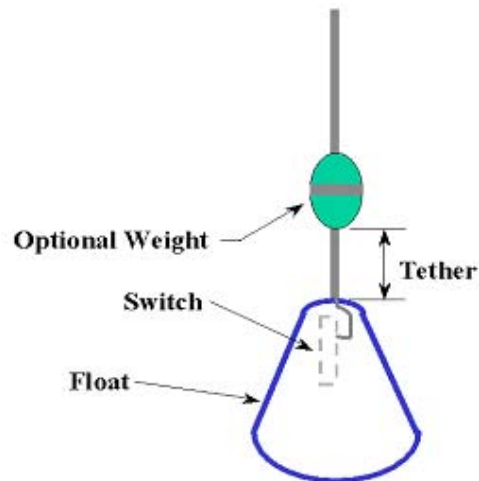
Figure 54: Components of a Simple Float Switch
