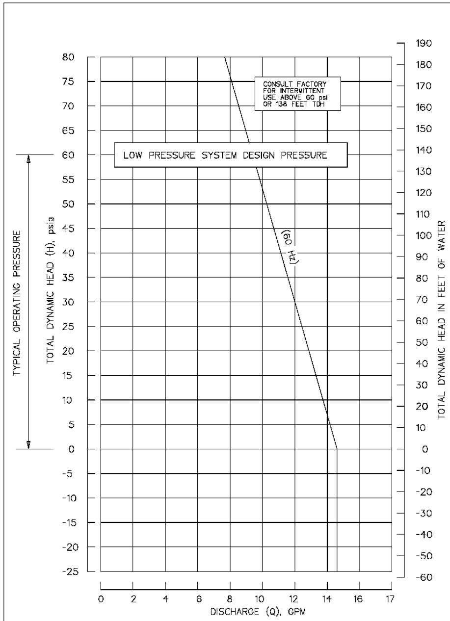
Environment One-semi-positive displacement, progressing cavity pump curve.
