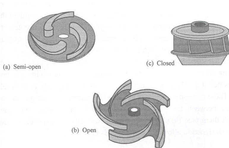
Figure 2 Impeller Designs
