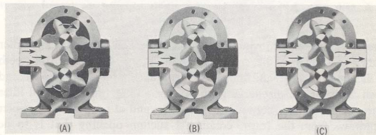
Fig. 2. Movement of a liquid through a gear-type hydraulic pumps: (A) Liquid entering the pump; (B) Liquid being carried between the teeth of the gears; and (C) Liquid being forced into the discharge line.
