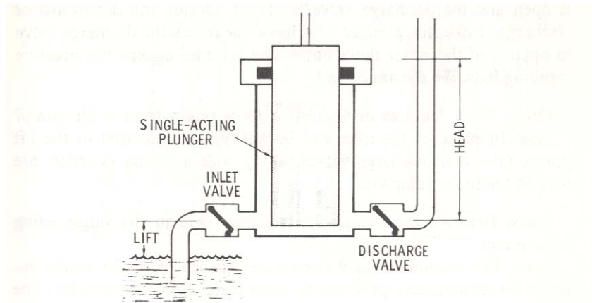
Fig. 6. Basic construction of a single-acting plunger-type force pump.
