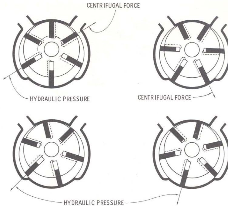
Figure 4 Rotary Vane Pump
