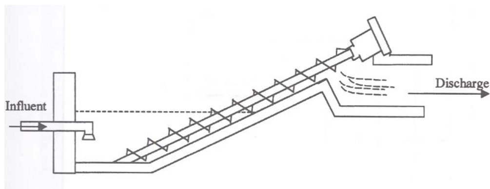
Figure 5 Screw Pump
