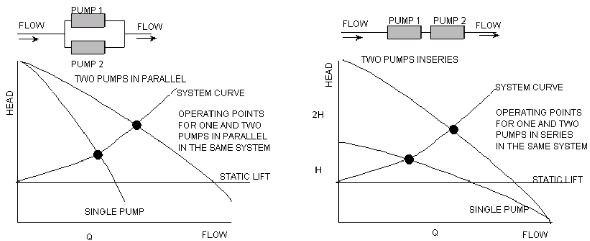
Figure 8 Pumps in Parallel and Series in a System
